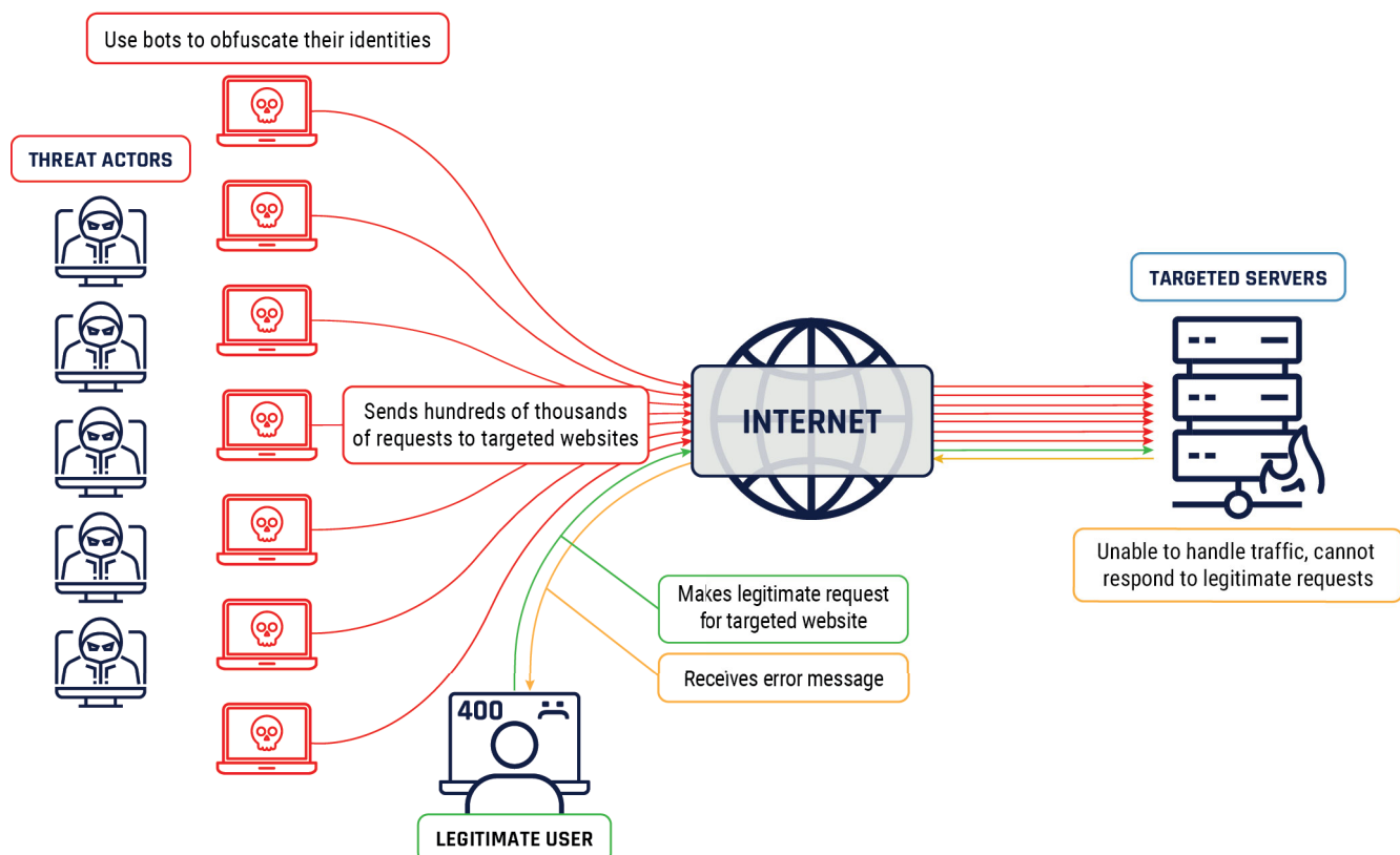
Figure 2: Distributed denial of service
