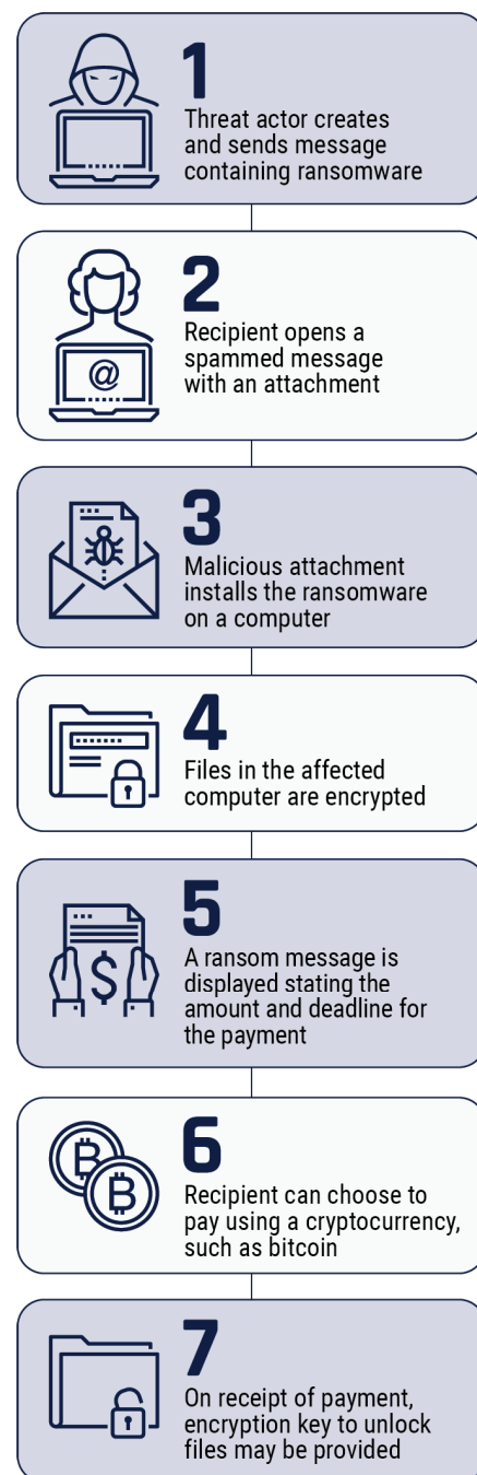
Figure 5: Ransomware
