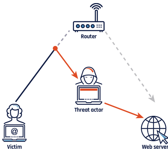
Figure 3: Person-in-the-middle
